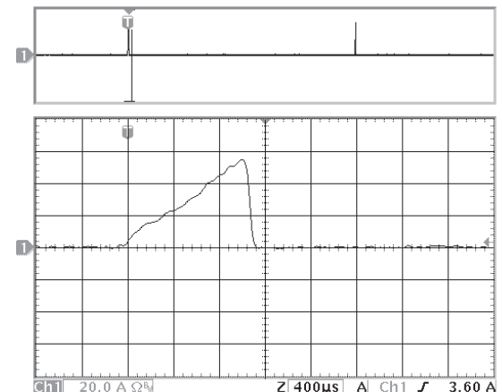
Figure 18: Load current (20A/div) as a function of time when the converter attempts to turn on into a 10 \text{ m}\Omega short circuit. Top trace (2.5ms/div) is an expansion of the on-time portion of the bottom trace.
