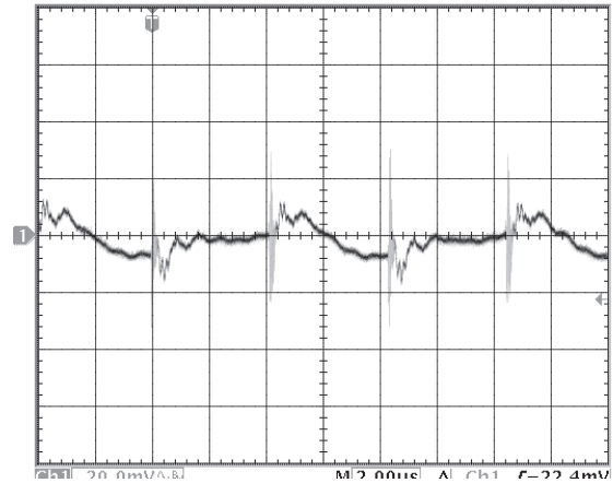
Figure 16: Output voltage ripple at nominal input voltage and rated load current (20 mV/div). Load capacitance: 1 \mu\text{F} ceramic capacitor and 10 \mu\text{F} tantalum capacitor. Bandwidth: 20 MHz. (See Figure 13)
