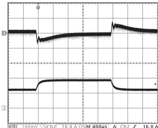
Figure 11: Output voltage response to step-change in load current (50%-75%-50% of I_{out(max)} ; dI/dt = 0.1A/\mu s ). Load cap: 10µF, 100 mΩ ESR tantalum cap and 1µF ceramic cap. Ch 1: V_{out} (100mV/div), Ch 2: I_{out} (10A/div).
