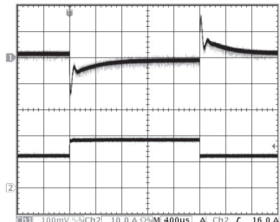
Figure 12: Output voltage response to step-change in load current (50%-75%-50% of I_{out(max)} ; dI/dt = 5A/\mu s ). Load cap: 470µF, 30 mΩ ESR tantalum cap and 1µF ceramic cap. Ch 1: V_{out} (100mV/div), Ch 2: I_{out} (10A/div).
