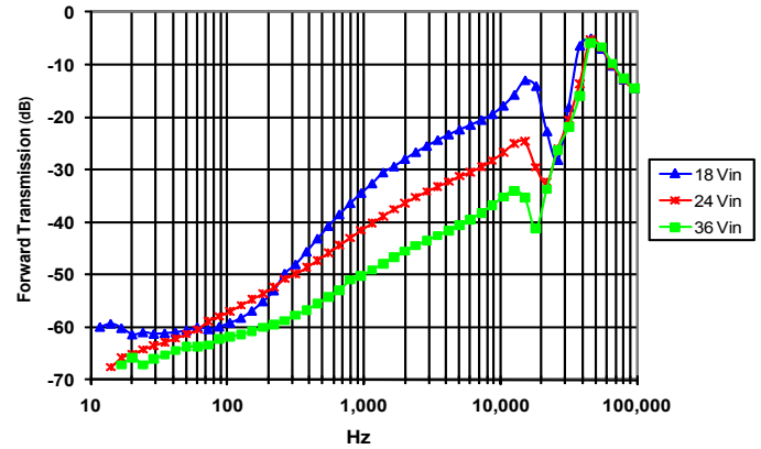
Figure 20: Magnitude of incremental forward transmission ( FT = v_{out}/v_{in} ) for minimum, nominal, and maximum input voltage at full rated power.
